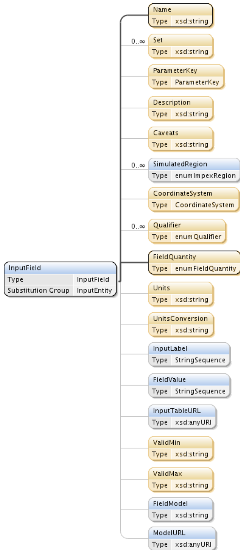
Figure 13 - InputField element
