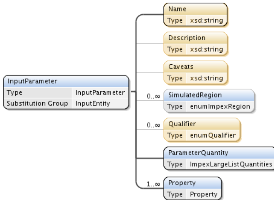
Figure 11 - InputParameter element
